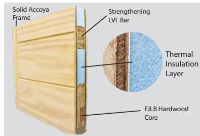
Patented CLPF Construction
