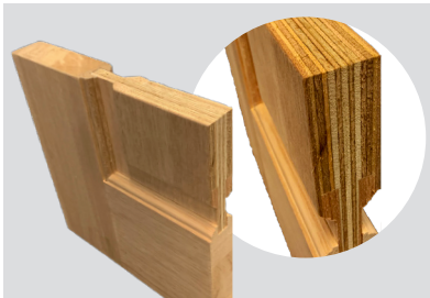
11 Ply Panel Construction
